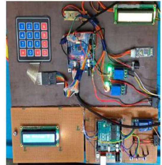
Figure 2: Circuit Board
